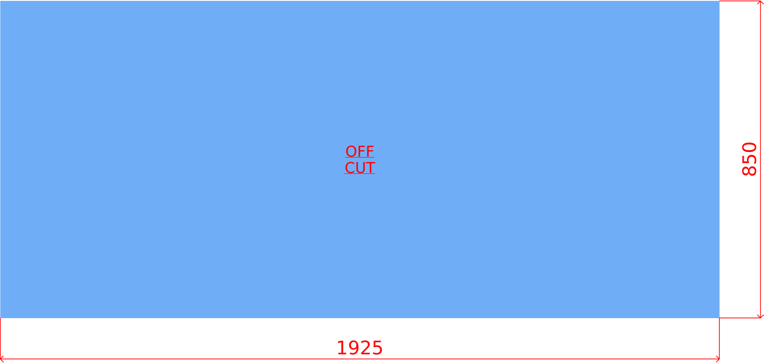
Offcut - Maple (WS-WO-3-960-40-MAPL) Initial worktop blank - 1925mm / 850mm / 40mm
